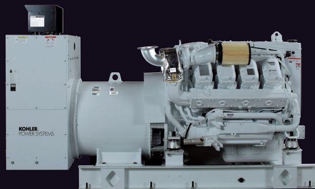
400EFOZC 400 kW
